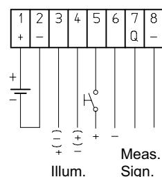
Anschluss Taster an Auxiliary
